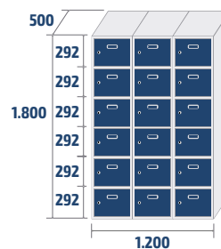
ECOB-40/3 PRO 74,3kg · 1,08m 3
